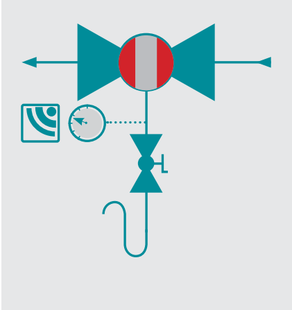
Type DBI-B
