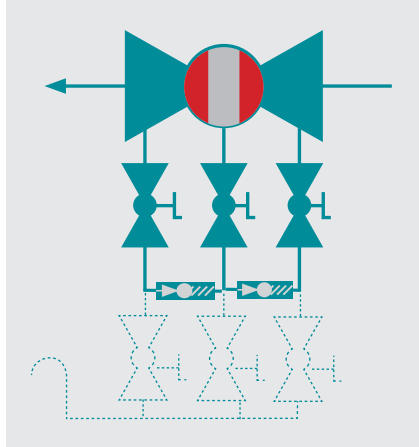
Type DBI-TR2
