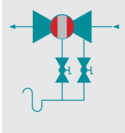
Type DBI-B&I
