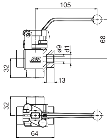
Type MGZ-24 with female thread
